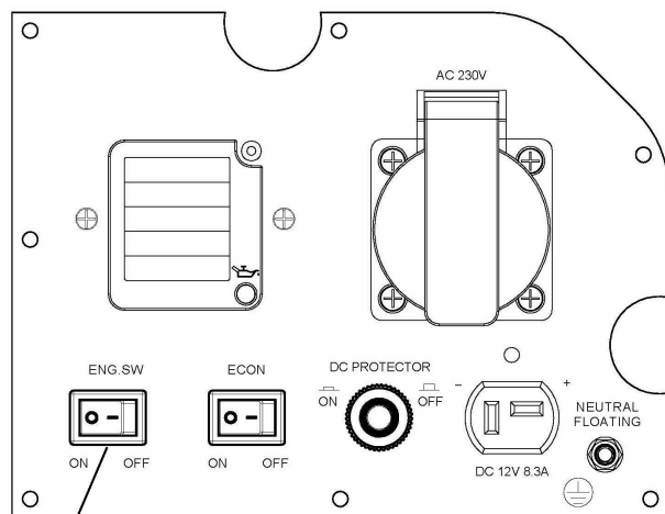
Engine switch
