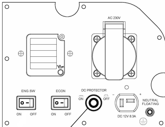
DC protector
