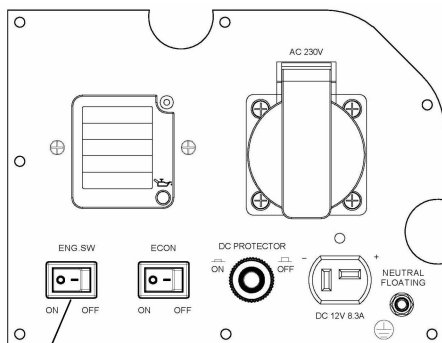
Engine switch
